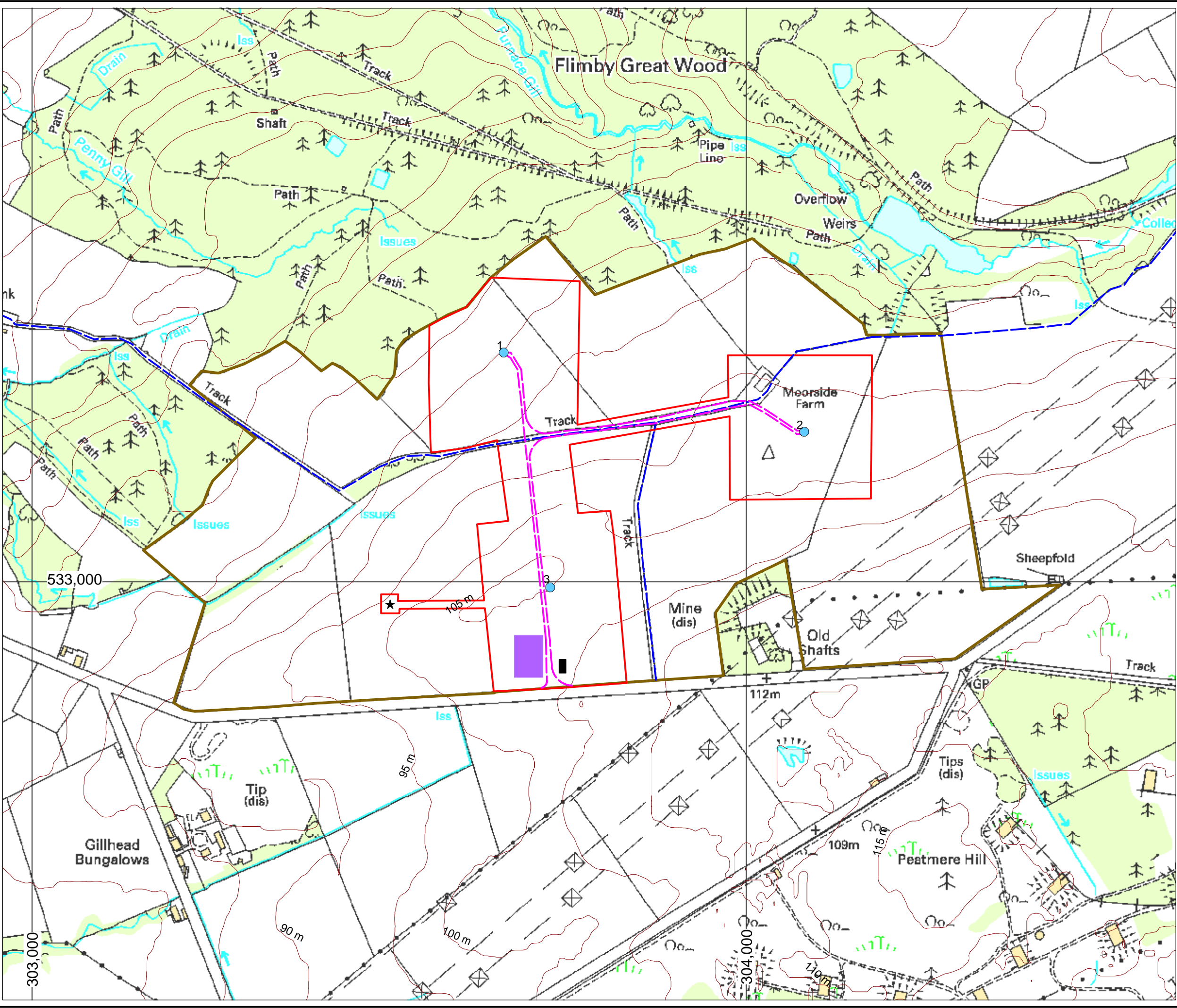
Figure 2 Site Layout & Application Boundary
